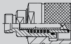
Pipe coupling
